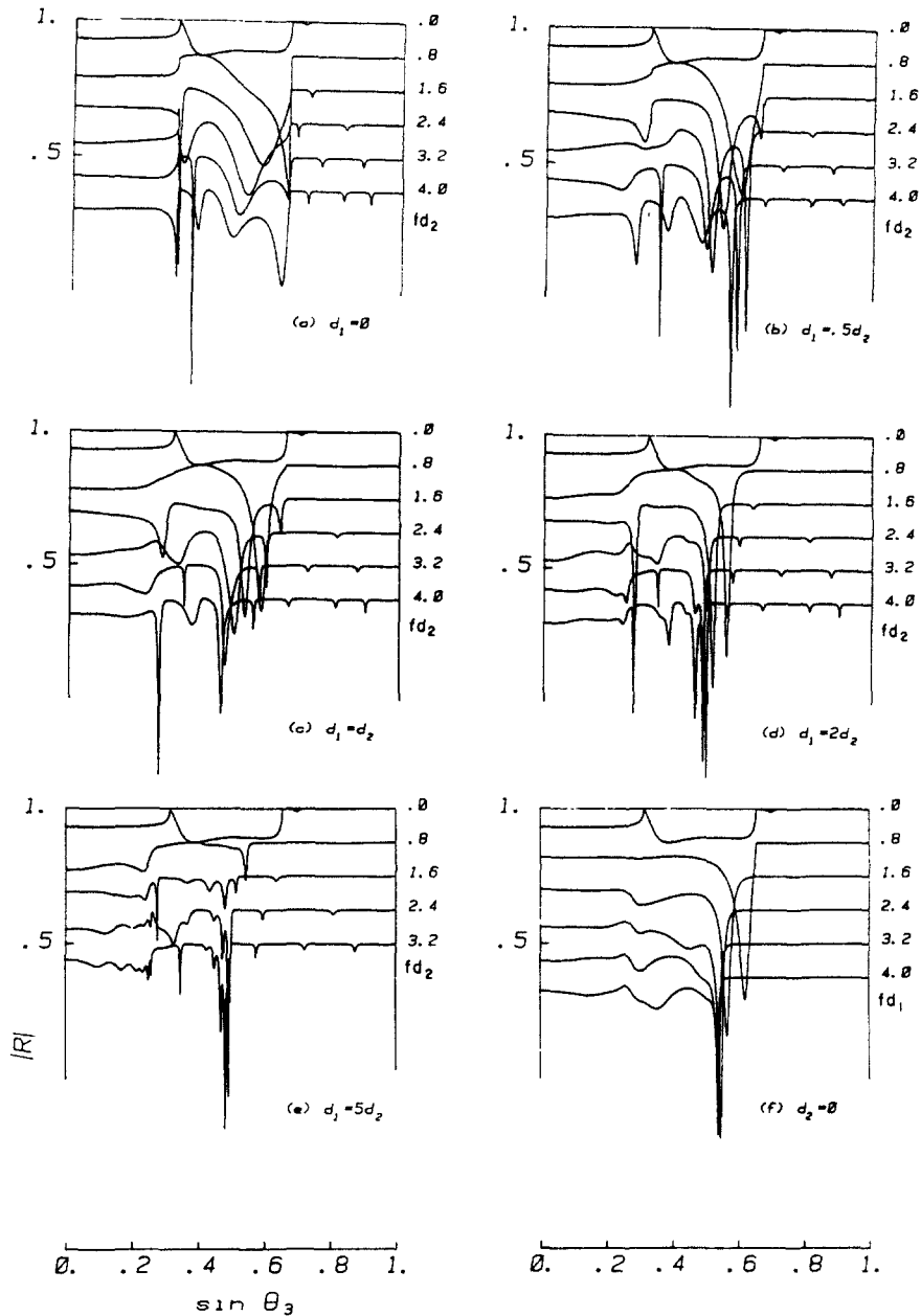
Fig. 4. Dependence of plane wave reflection coefficient on the ratio of layer thicknesses and a frequency-thickness parameter. fd_1 and fd_2 have units of MHz · mm. Only the top curve is properly positioned with respect to the ordinate axis in each graph, i.e. |R| = 1 at \sin \theta_3 = 1 for all curves. The structure is as shown in Fig. 3.
